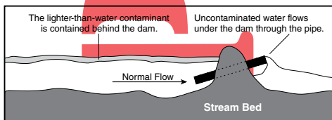
Underflow Dam (side view)
