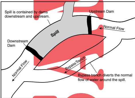
The normal flow of water is diverted around a spill (top view).
