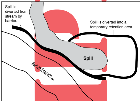
The spill is diverted away from the stream and into a temporary retention area (top view).
